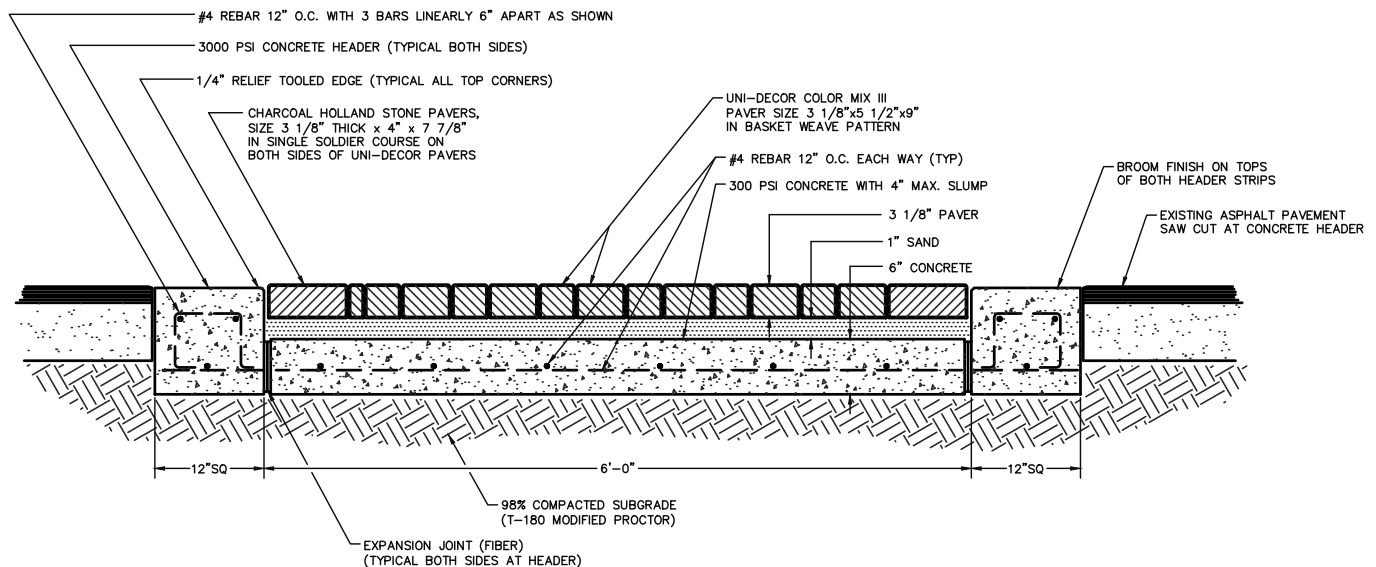
TYPICAL CROSSWALK PAVER DETAIL – SECTION A-A
