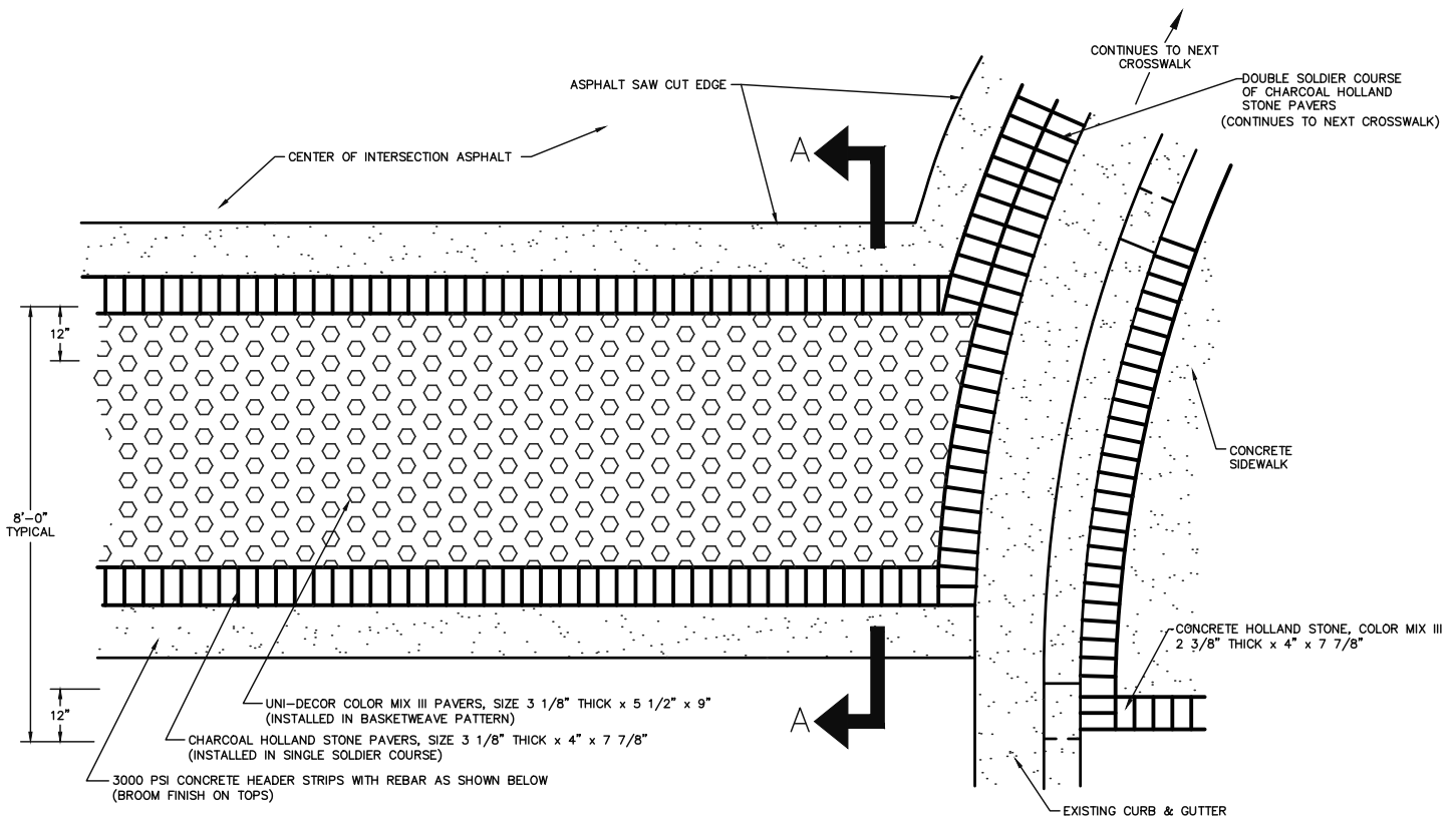
TYPICAL CROSSWALK PAVER DETAIL – PLAN VIEW
