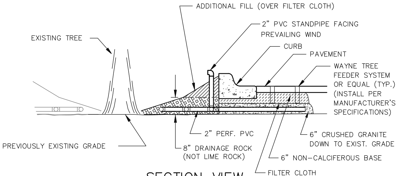
SECTION VIEW
