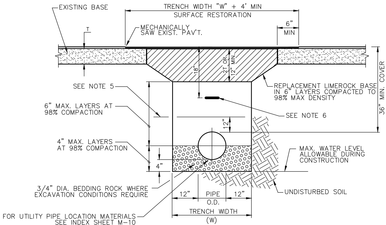
PAVEMENT CUT AND PATCH DETAIL
