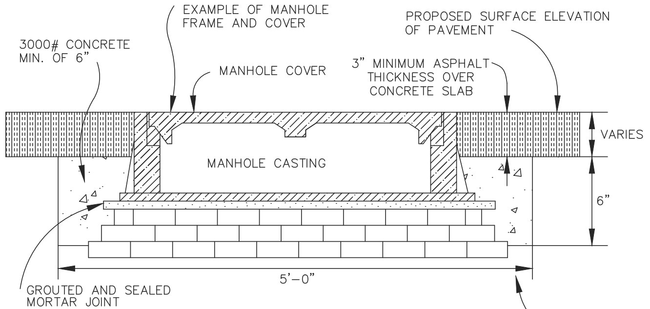
HALF SECTION
