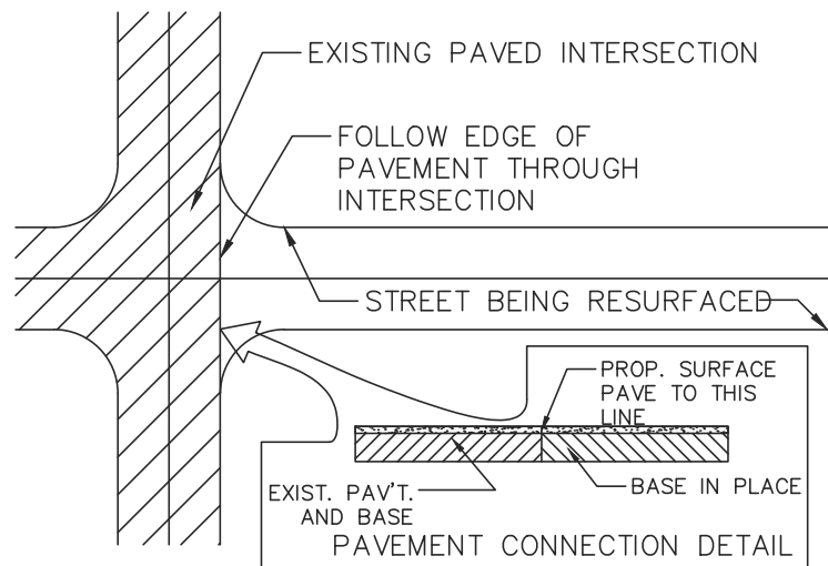
STANDARD DETAIL FOR PAVED INTERSECTION THICKNESS VARIES
